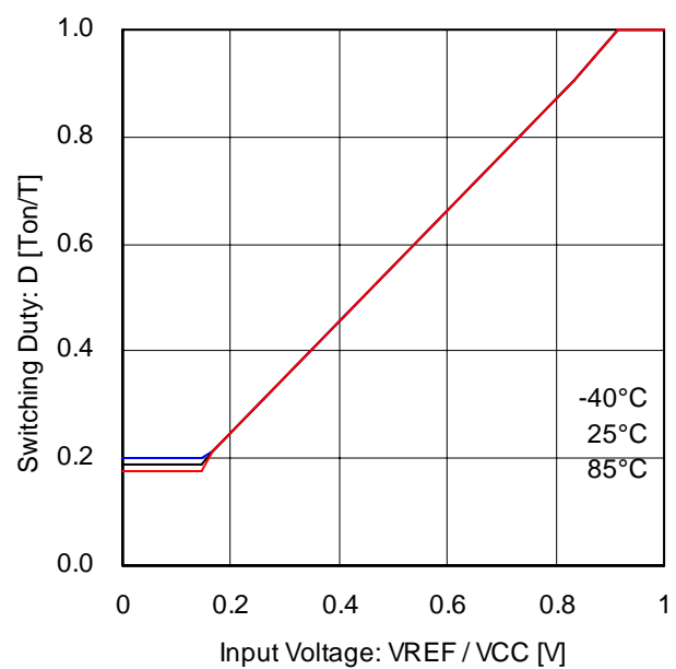
Fig.14 V_{REF} - DUTY( V_{CC}=12V )
