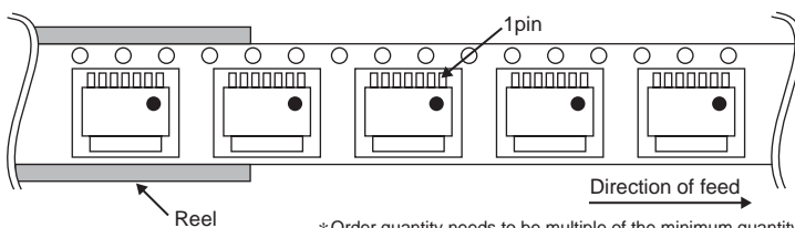
Tape Embossed carrier tape Quantity 2000pcs Direction of feed TR ( The direction is the 1pin of product is at the upper right when you hold reel on the left hand and you pull out the tape on the right hand )
