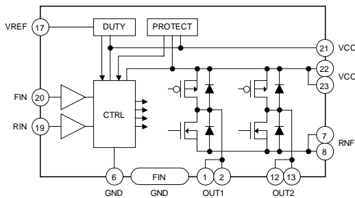
Fig.5 BD6222FP
