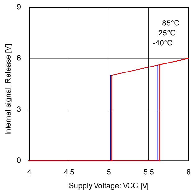
Fig.16 Under voltage lock out
