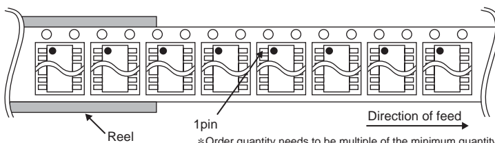
Tape Embossed carrier tape Quantity 2000pcs Direction of feed E2 ( The direction is the 1pin of product is at the upper left when you hold reel on the left hand and you pull out the tape on the right hand )
